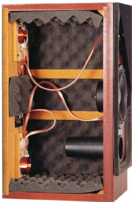
This cutaway of Image 3 MK II reveals many of the details contributing to the fine sound of Image of Australia speakers. Note the rigid bracings, separate crossover network boards, audiophile speaker cable internal wiring, Solen capacitors and the quality of the cabinet work. All these features contribute greatly to the final sound quality.
