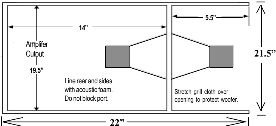
One possible version of Audax Subwoofer (view through centerline)
