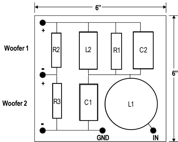
Left / Right Speaker Woofer Crossover Layout (2 x Boards)
