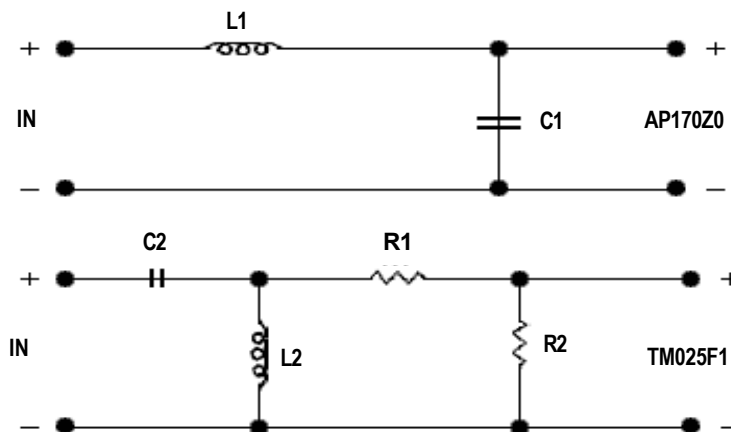
Surround Speaker Crossover Network
