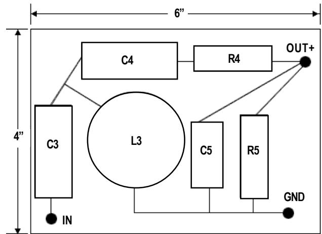
Left / Right Speaker Tweeter Crossover Layout (2 x Boards)
