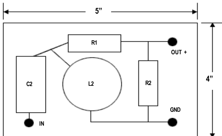
Surround Speaker Tweeter Crossover Layout (2 x Boards)
