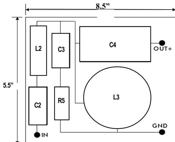
Crossover Layout for Center Channel Midrange (1 x Board)
