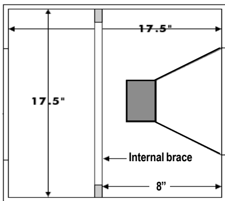
Subwoofer 1 (revised for HT300Z2)
