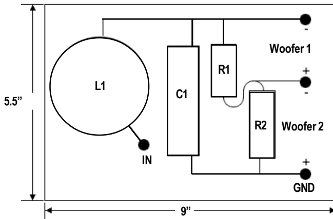
Center Channel Woofer Crossover Layout (Note: Woofer polarity is reversed.) (1 x Board)
