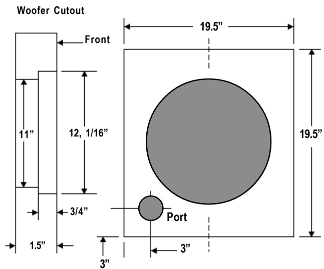
View of Woofer Baffle
