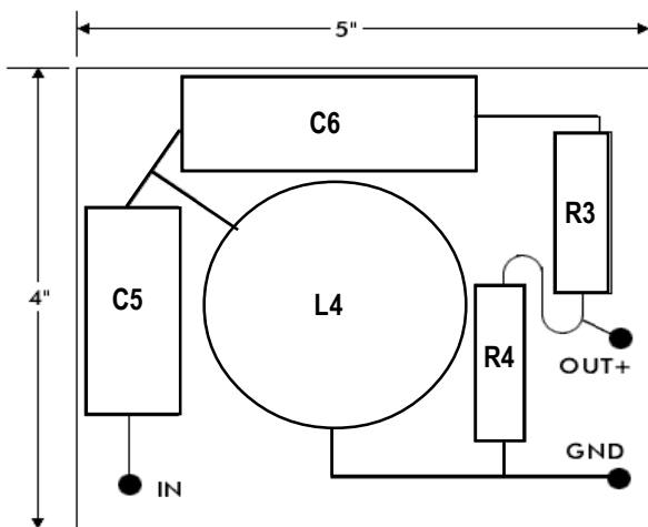
Crossover Layout for Center Channel Tweeter (1 x Board)
